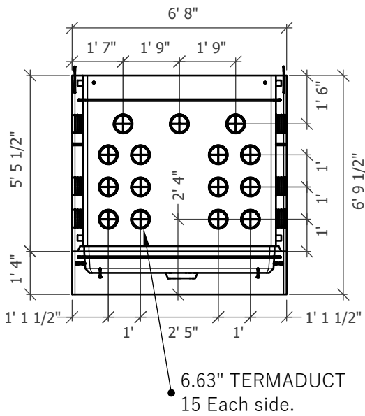
END VIEW
